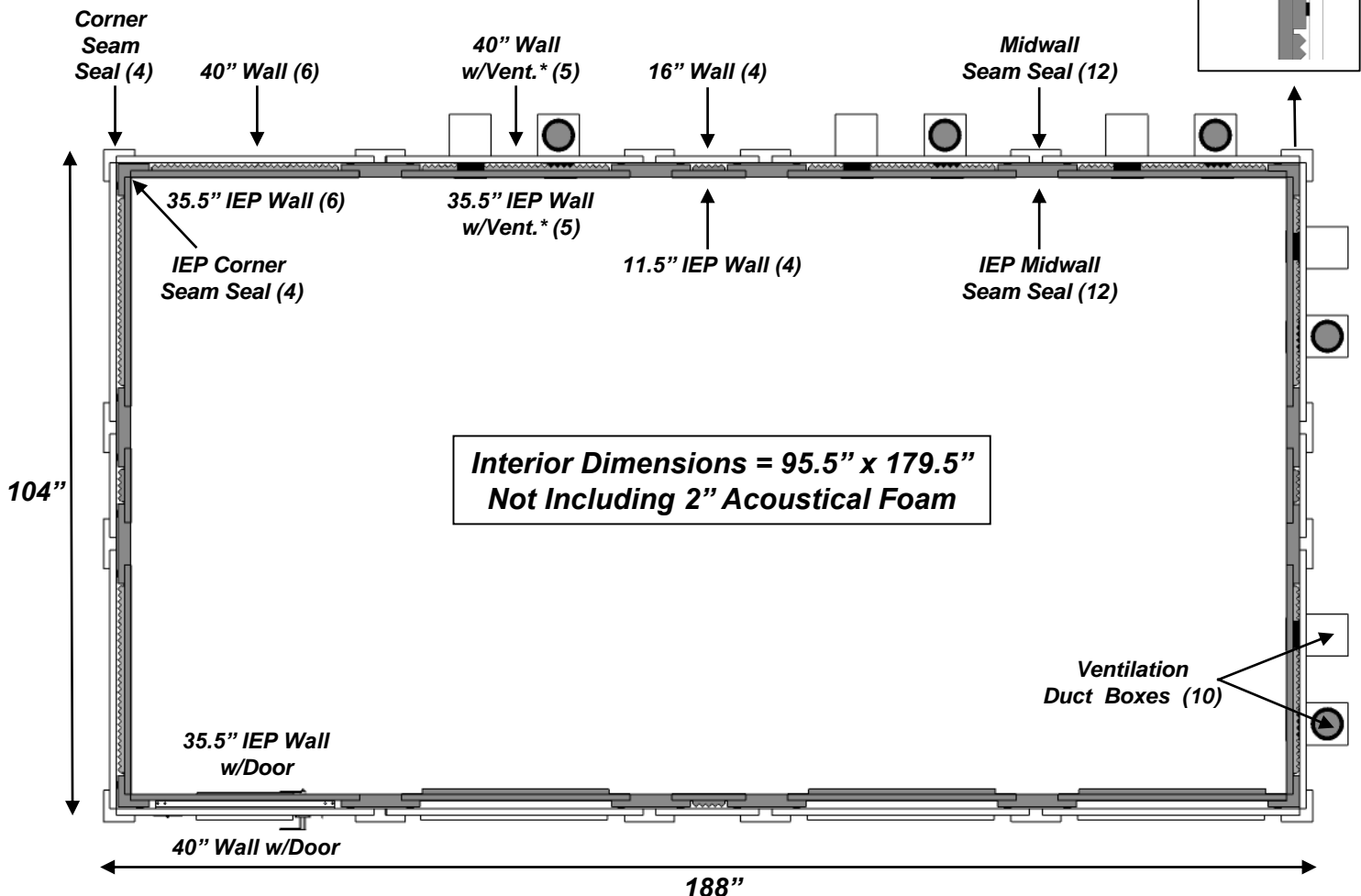
Top-Down represents typical configuration
