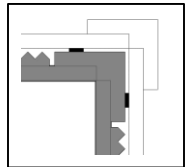
Enlarged view of corner seam seals
