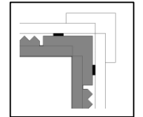
Enlarged view of corner seam seals
