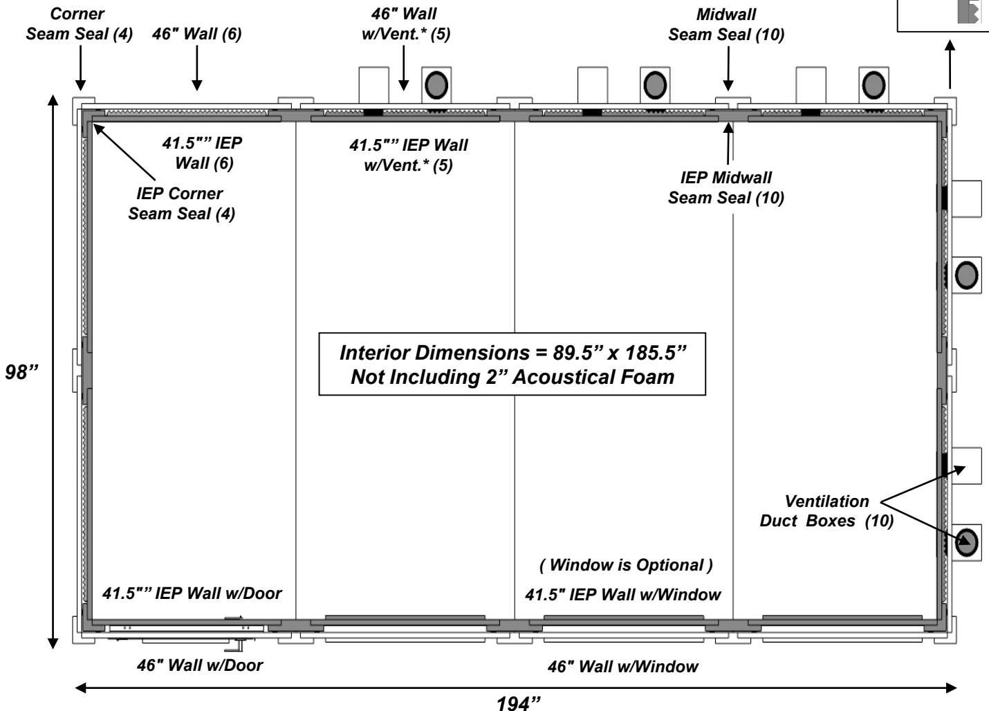
Top-Down represents typical configuration
